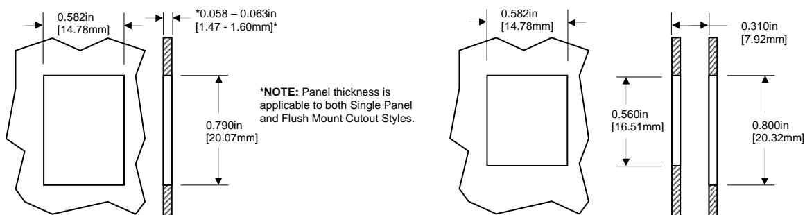
Single Panel Cutout
