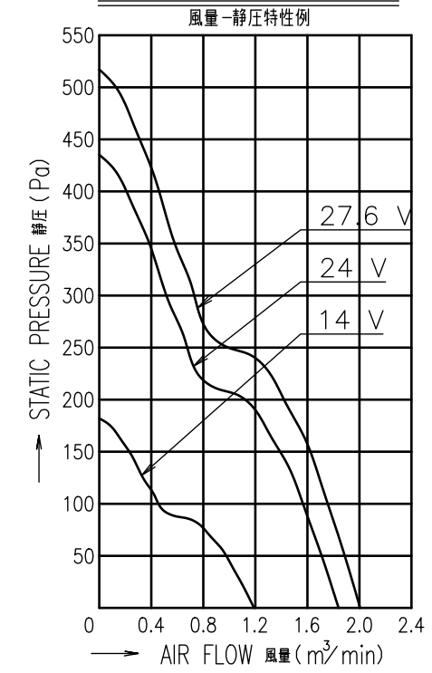
PERFORMANCE CURVES
