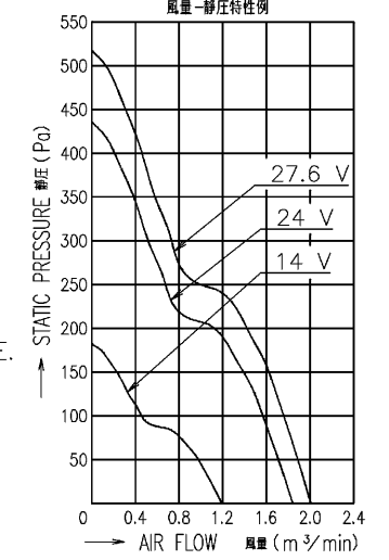
PERFORMANCE CURVES 風量-静圧特性例
