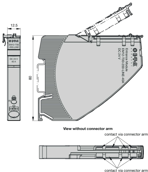
EM12-T00-200-LINE-40A supply module centre/LINE, LINE separated
