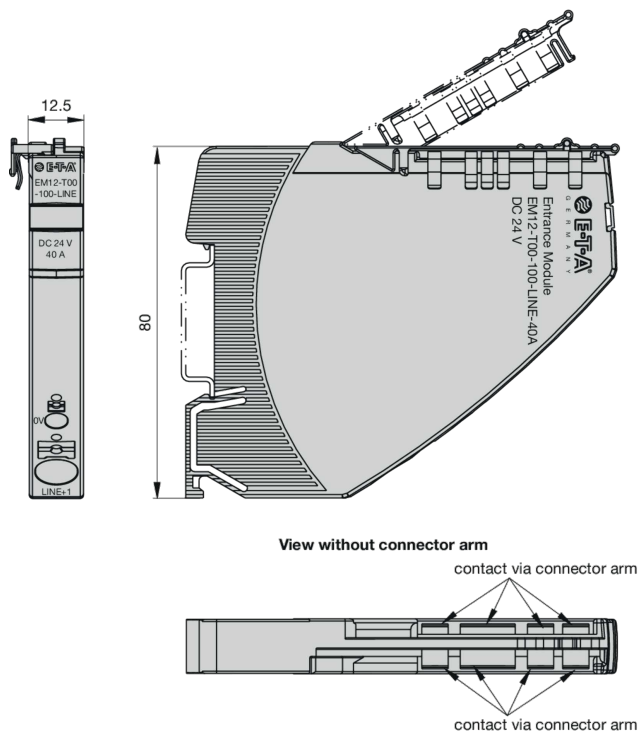
EM12-T00-100-LINE-40A supply module centre/right – LINE, LINE connected
