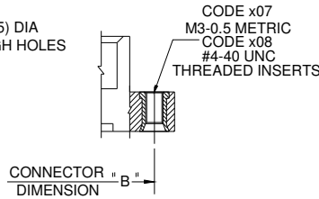
CONNECTOR "B" DIMENSION MOUNTING OPTION CODES x07 & x08 (THREADED INSERTS)
