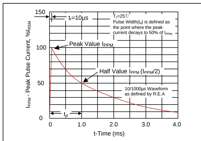
Figure 2. 10/1000 \mu\text{s} Pulse Waveforms
