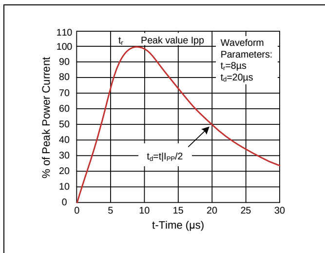
Figure 3. 8/20 \mu\text{s} Pulse Waveforms
