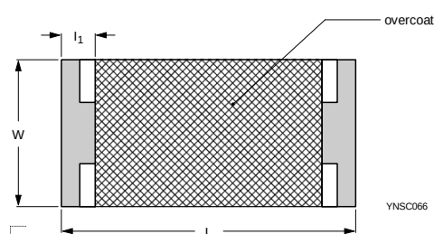
Fig. 5 Chip resistor outlines
