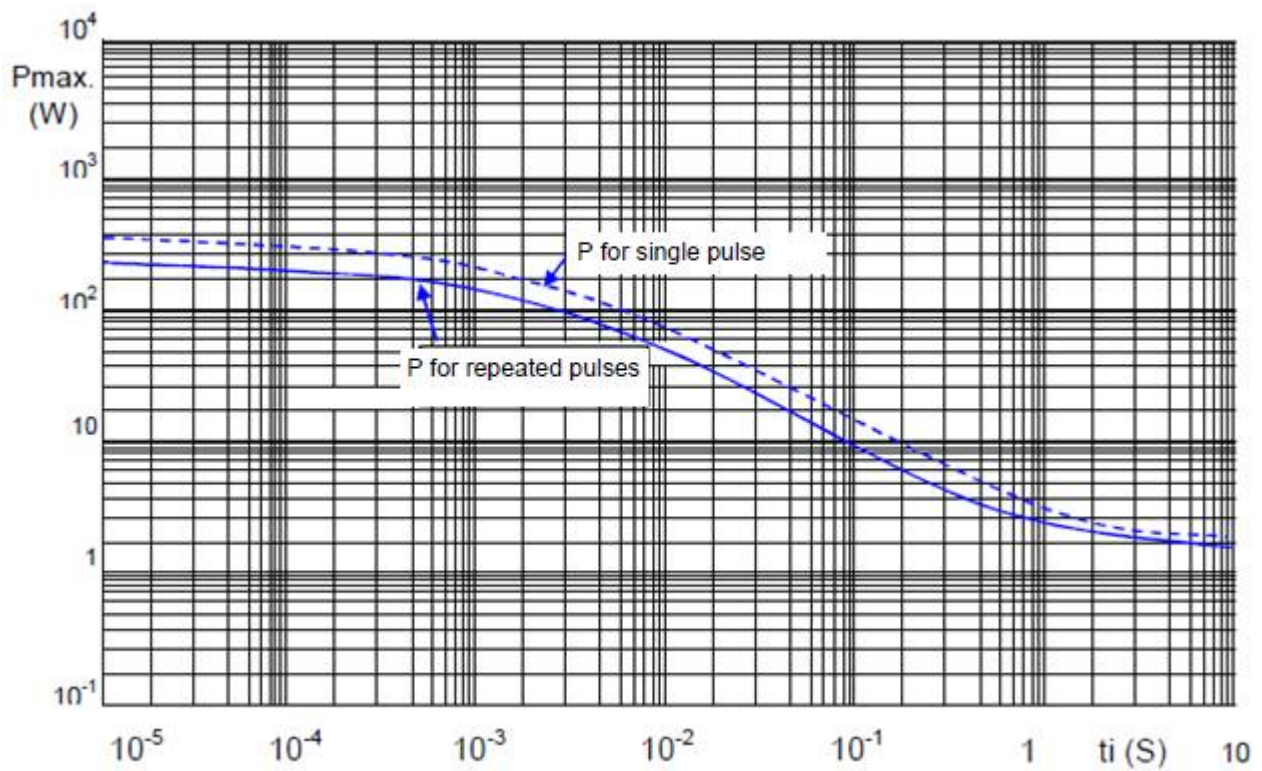
RSF200 Series: P_{max} : Maximum permissible peak pulse power t_i : Pulse duration
