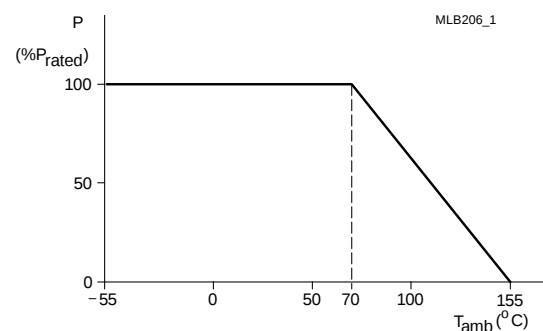
Fig. 6 Maximum dissipation ( P_{max} ) in percentage of rated power as a function of the operating ambient temperature ( T_{amb} )
