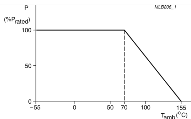
Fig. 10 Maximum dissipation ( P_{max} ) in percentage of rated power as a function of the operating ambient temperature ( T_{amb} )
