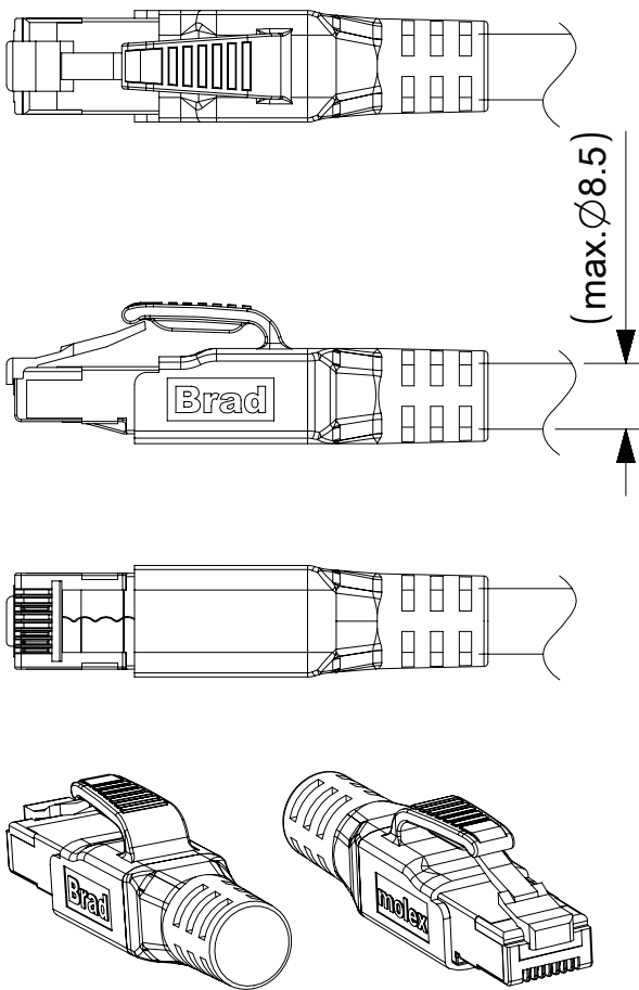
OVERMOLD VIEW FOR CABLES O.D.≥6.7mm
