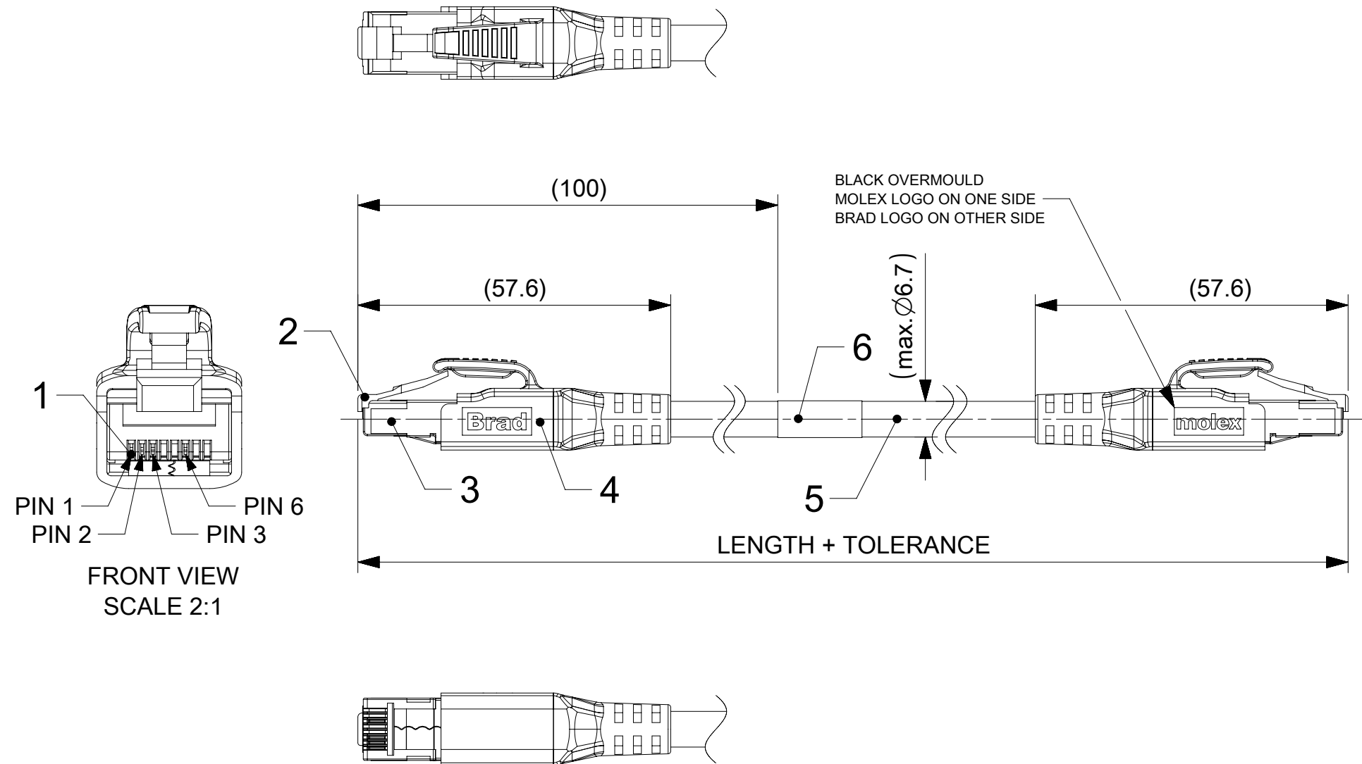
OVERMOLD VIEW FOR CABLES O.D.≤6.7mm
