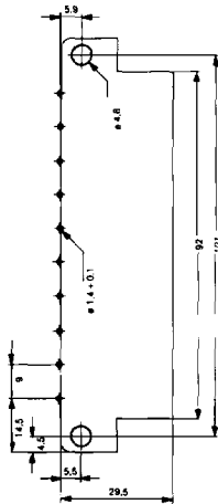
STV 4/10 S with soldering lug
