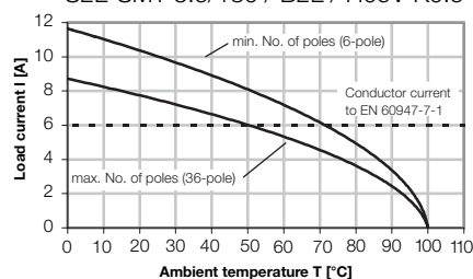
S2L-SMT 3.5/180 / B2L / H05V-K0.5
