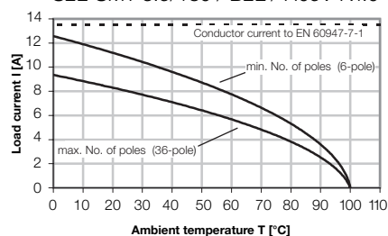
S2L-SMT 3.5/180 / B2L / H05V-K1.0
