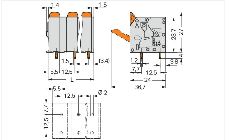
Dimensions in mm L = (\text{pole no.} - 1) \times \text{pin spacing} + 9 \text{ mm}
