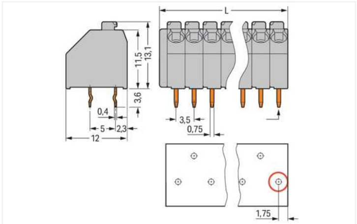
Dimensions in mm L = (\text{pole no.} \times \text{pin spacing}) + 1.5 \text{ mm} First solder pin, front right (red circle)
