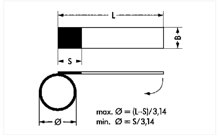
Dimensions in mm Dimensions of self-laminating label
