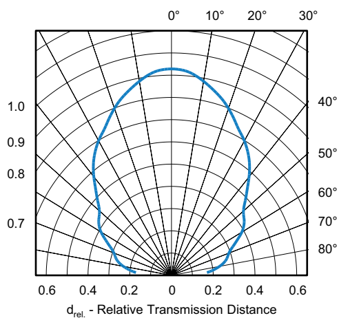
Fig. 11 - Horizontal Directivity
