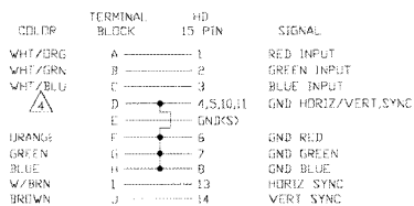
WIRING DIAGRAM
