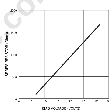
SERIES LIMIT BIAS RESISTOR VS BIAS VOLTAGE FIGURE 8 (See Note 1)
