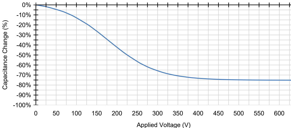
VCC Characterization
