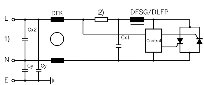
Interference suppression with resistive load, 2-stage
