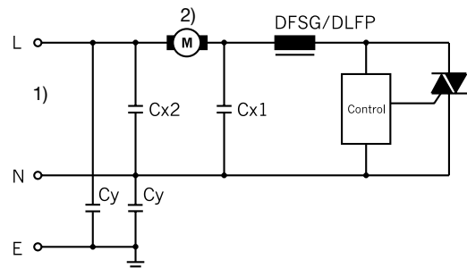
Interference suppression with inductive load
