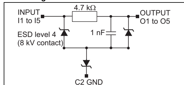
Figure 2. Functional schematic
