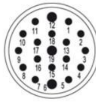
Insert Pin Mating View
