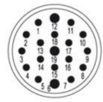
Insert Socket Mating View
