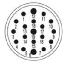
Insert Socket Mating View
