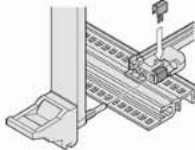
Optional ESD clip for alignment pin
