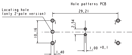
Locating hole only version 2 NO/2 NC
