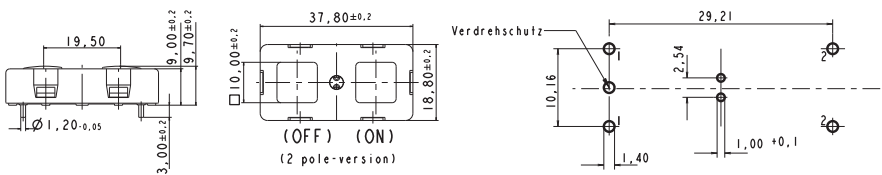
PCB footprint
