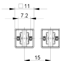
Illustration with 2 LED OSRAM LO M676-Q1R1-24
