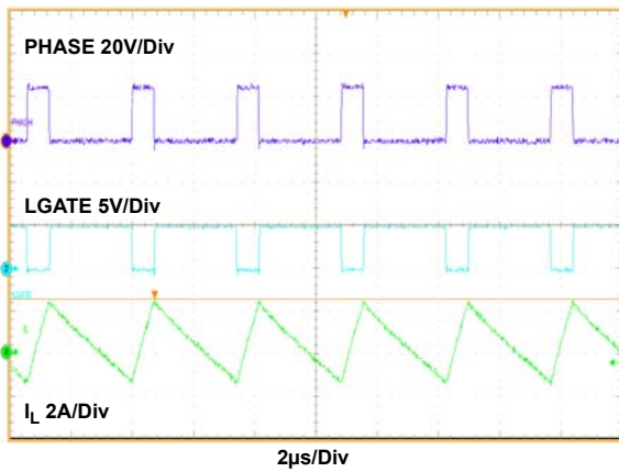
Figure 15. PHASE, LGATE, and Inductor Current Waveforms, I_0 = 0A
