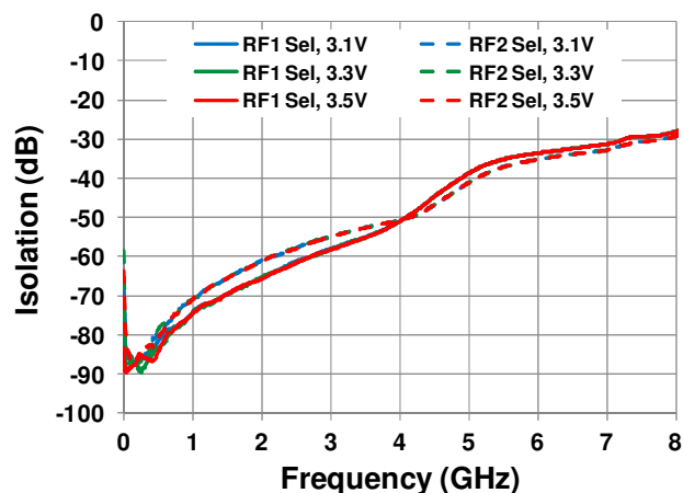
Isolation vs. Voltage [RF1 → RF2, RF2 → RF1]
