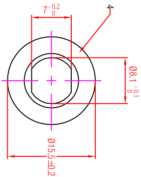
Washer
