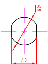
Panel Cut Out (Rear Side)
