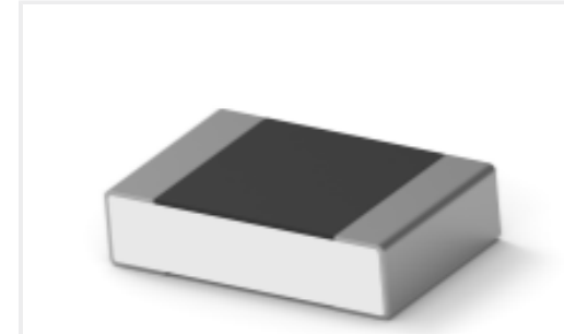
TE Part #1-2176379-3 RQ 0805 143R 0.1% 10PPM 5K RL RT 2R
