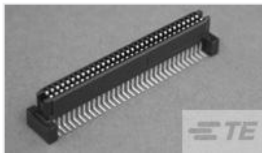
TE Part #1-5146894-1 1FHR,64,50A/S,S,C,S11,12
