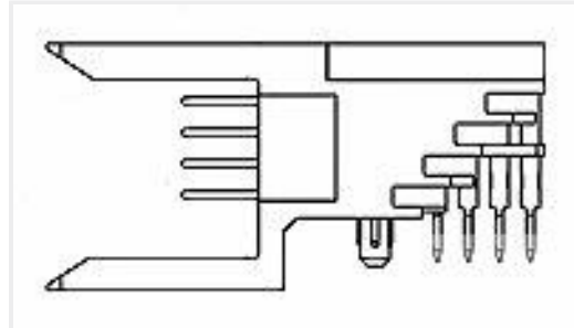
TE Part #5223514-2 2MM FB,IS,ASY,048,SIG,HDR,SL
