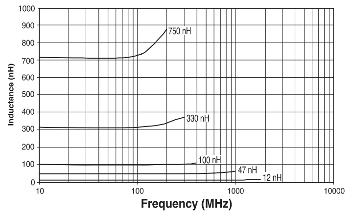
Typical Inductance vs Frequency
