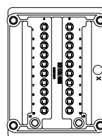
BOTTOM VIEW 1530X-1-X-X FUSE BASE
