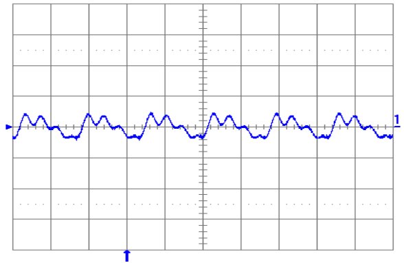
Fig. 2.0V.5: Output voltage ripple (20mV/div.) at full rated load current into a resistive load with external capacitance 100 \mu F ceramic + 1 \mu F ceramic and V_{in} = 12 V for V_{out} = 2.0 V. Time scale: 2 \mu s/div.
