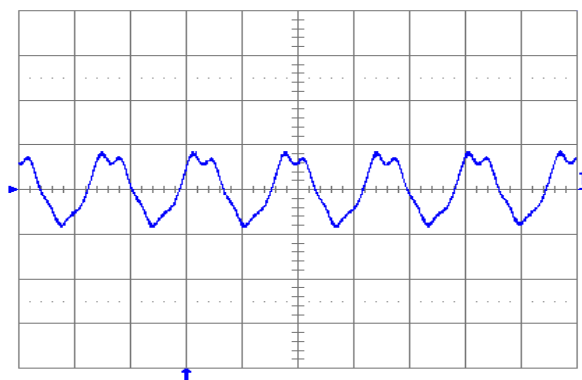
Fig. 5.0V.5: Output voltage ripple (20 mV/div.) at full rated load current into a resistive load with external capacitance 100 \mu F ceramic + 1 \mu F ceramic and V_{in} = 12 V for V_{out} = 5.0 V. Time scale: 2 \mu s/div.
