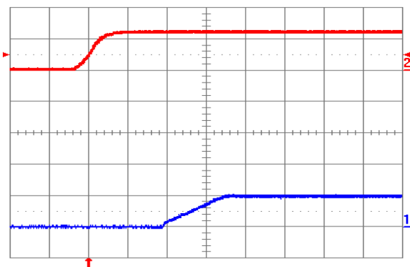
Fig. 1.0V.4: Turn-on transient for V_{out} = 1.0 V with application of V_{in} at full rated load current (resistive) and 100 \mu F external capacitance at V_{in} = 12 V. Top trace: V_{in} (10 V/div.); Bottom trace: output voltage (1 V/div.); Time scale: 2 ms/div.
