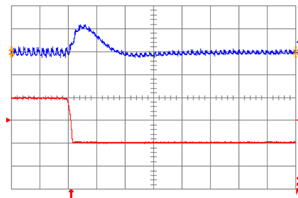
Fig. 3.3V.7: Output voltage response for V_{out} = 3.3 V to negative load current step change from 20 A to 10 A with slew rate of -5A/ \mu s at V_{in} = 12 V. Top trace: output voltage (200 mV/div.); Bottom trace: load current (5 A/div.). C_o = 100 \mu F ceramic. Time scale: 20 \mu s/div.
