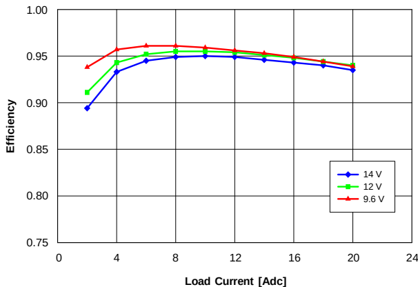
Fig. 5.0V.2: Efficiency vs. load current and input voltage for V_{out} = 5.0 V converter mounted vertically with air flowing at a rate of 200 LFM (1 m/s) and T_a = 25 °C.
