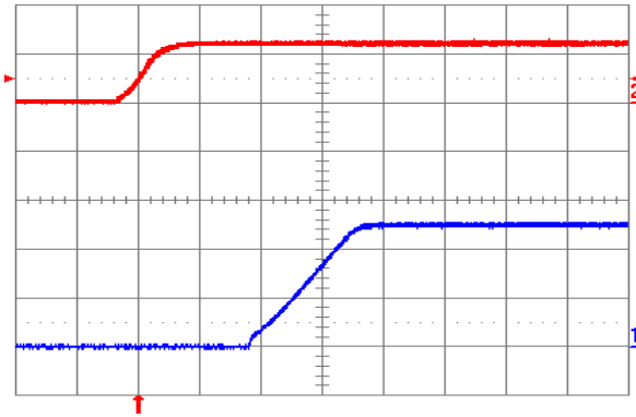
Fig. 2.5V.4: Turn-on transient for V_{out} = 2.5 V with application of V_{in} at full rated load current (resistive) and 100 \mu F external capacitance at V_{in} = 12 V. Top trace: V_{in} (10 V/div.); Bottom trace: output voltage (1 V/div.); Time scale: 2 ms/div.
