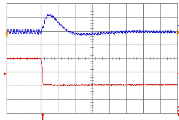
Fig. 5.0V.7: Output voltage response for V_{out} = 5.0 V to negative load current step change from 20 A to 10 A with slew rate of -5 A/ \mu s at V_{in} = 12 V. Top trace: output voltage (200 mV/div.); Bottom trace: load current (5 A/div.). C_o = 100 \mu F ceramic. Time scale: 20 \mu s/div.
