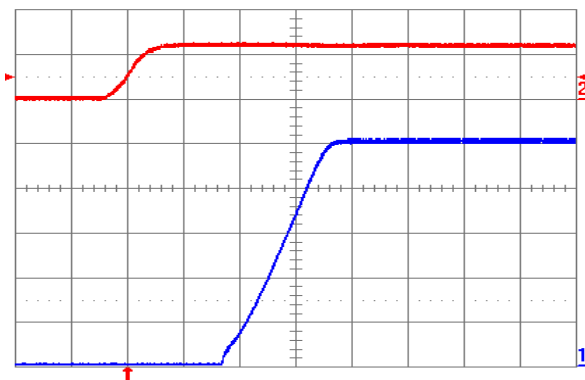
Fig. 5.0V.4: Turn-on transient for V_{out} = 5.0 V with application of V_{in} at full rated load current (resistive) and 100 \mu F external capacitance at V_{in} = 12 V. Top trace: V_{in} (10 V/div.); Bottom trace: output voltage (1 V/div.); Time scale: 2 ms/div.
