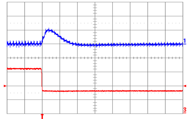
Fig. 2.0V.7: Output voltage response for V_{out} = 2.0 V to negative load current step change from 20 A to 10 A with slew rate of -5A/ \mu s at V_{in} = 12 V. Top trace: output voltage (200 mV/div.); Bottom trace: load current (5 A/div.). C_o = 100 \mu F ceramic. Time scale: 20 \mu s/div.
