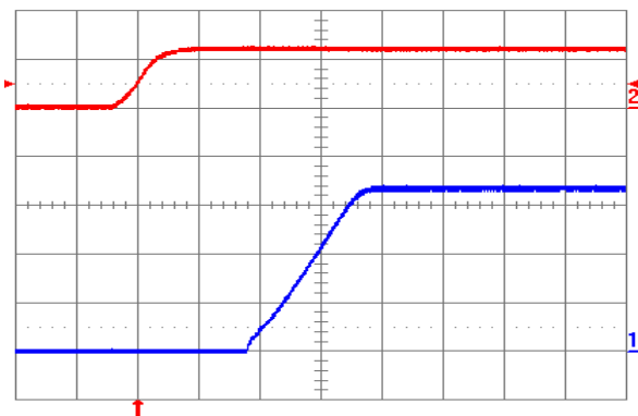
Fig. 3.3V.4: Turn-on transient for V_{out} = 3.3 V with application of V_{in} at full rated load current (resistive) and 100 \mu F external capacitance at V_{in} = 12 V. Top trace: V_{in} (10 V/div.); Bottom trace: output voltage (1 V/div.); Time scale: 2 ms/div.
