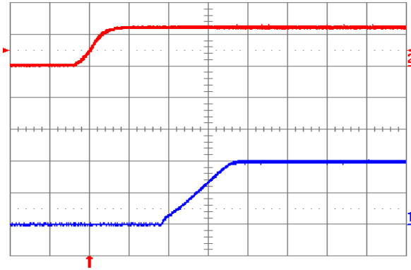
Fig. 2.0V.4: Turn-on transient for V_{out} = 2.0 V with application of V_{in} at full rated load current (resistive) and 100 \mu F external capacitance at V_{in} = 12 V. Top trace: V_{in} (10 V/div.); Bottom trace: output voltage (1 V/div.); Time scale: 2 ms/div.
