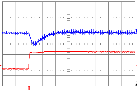
Fig. 2.0V.6: Output voltage response for V_{out} = 2.0 V to positive load current step change from 10 A to 20 A with slew rate of 5 A/ \mu s at V_{in} = 12 V. Top trace: output voltage (200 mV/div.); Bottom trace: load current (5 A/div.). C_o = 100 \mu F ceramic. Time scale: 20 \mu s/div.
