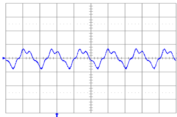
Fig. 3.3V.5: Output voltage ripple (20 mV/div.) at full rated load current into a resistive load with external capacitance 100 \mu F ceramic + 1 \mu F ceramic and V_{in} = 12 V for V_{out} = 3.3 V. Time scale: 2 \mu s/div.
