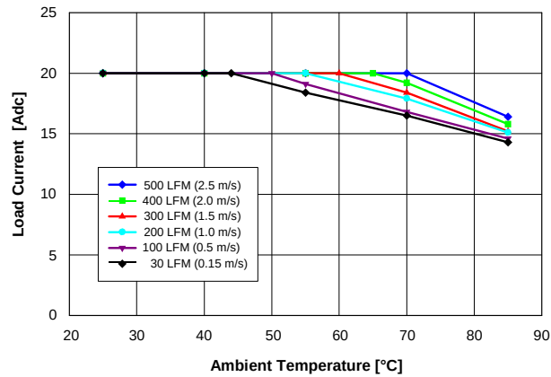
Fig. 1.0V.1: Available load current vs. ambient temperature and airflow rates for V_{out} = 1.0 V converter mounted vertically with V_{in} = 12 V, and maximum MOSFET temperature \leq 120 °C.
