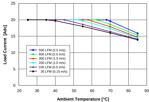
Fig. 2.0V.1: Available load current vs. ambient temperature and airflow rates for Vout = 2.0 V converter mounted vertically with Vin = 12 V, and maximum MOSFET temperature ≤ 120 °C.
