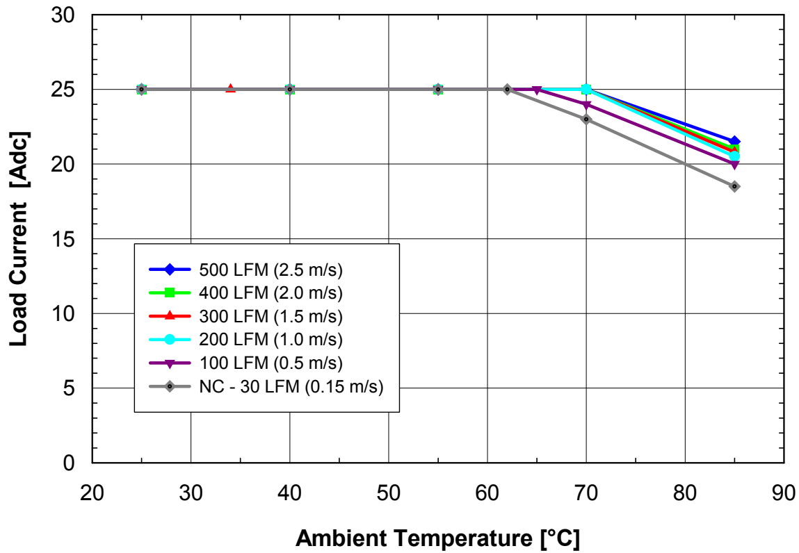
Figure 1. Available load current vs. ambient air temperature and airflow rates for SSQE48T25015 converter mounted vertically with air flowing from pin 1 to pin 3, Vin = 48 V. Note: NC – Natural convection
