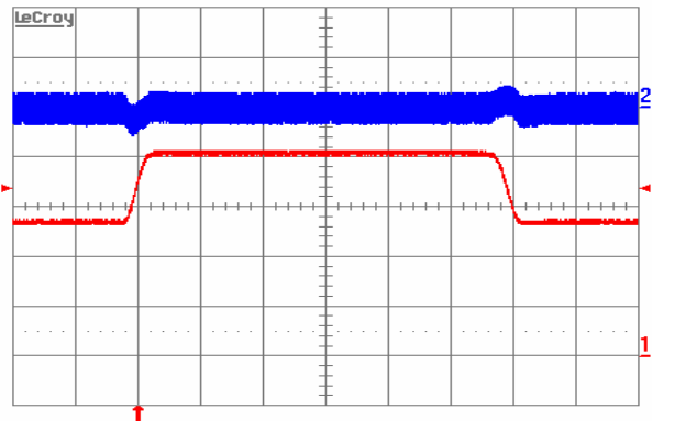
Figure 8. Output voltage response to load current step-change (12.5A-18.75A-12.5A) at V_{in}=48\text{V} . Top trace: output voltage (100mV/div.). Bottom trace: load current (5A/div.). Current slew rate: 0.1A/ \mu\text{s} . C_o=1\mu\text{F cer}+10\mu\text{F tant} . Time scale: 0.2ms/div.
