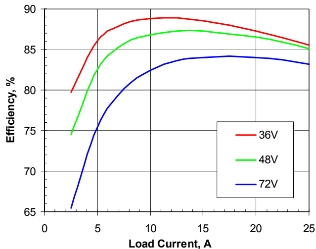
Figure 2. Efficiency vs. load current and input voltage for SSQE48T25015 converter mounted vertically with air flowing from pin 1 to pin 3 at a rate of 300 LFM (1.5 m/s) and Ta=25°C.
