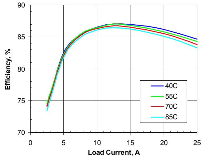
Figure 3. Efficiency vs. load current and ambient temperature for SSQE48T25015 converter mounted vertically with Vin=48V and air flowing from pin 1 to pin 3 at a rate of 200 LFM (1.0 m/s).
