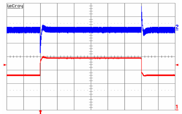
Figure 9. Output voltage response to load current step-change (12.5A-18.75A-12.5A) at V_{in}=48\text{V} . Top trace: output voltage (100 mV/div.). Bottom trace: load current (5A/div.). Current slew rate: 5A/ \mu\text{s} . C_o=470\mu\text{F POS}+1\mu\text{F cer} . Time scale: 0.2ms/div.
