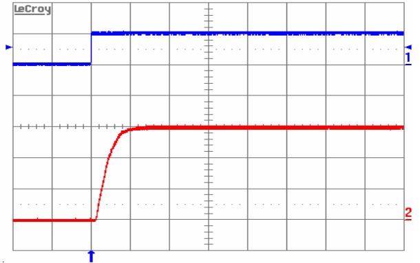
Figure 7. Turn-on transient at full rated load current (resistive) plus 30,000 \mu\text{F} at V_{in} = 48\text{ V} , triggered via ON/OFF pin. Top trace: ON/OFF signal (5 V/div.). Bottom trace: Output voltage (0.5 V/div.). Time scale: 5 ms/div.
