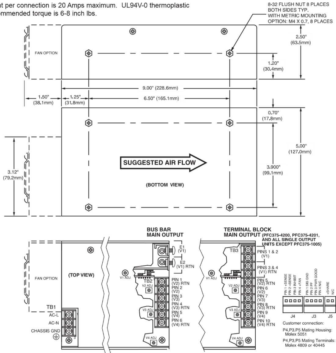
Figure 1. Mechanical Drawing PFC375
