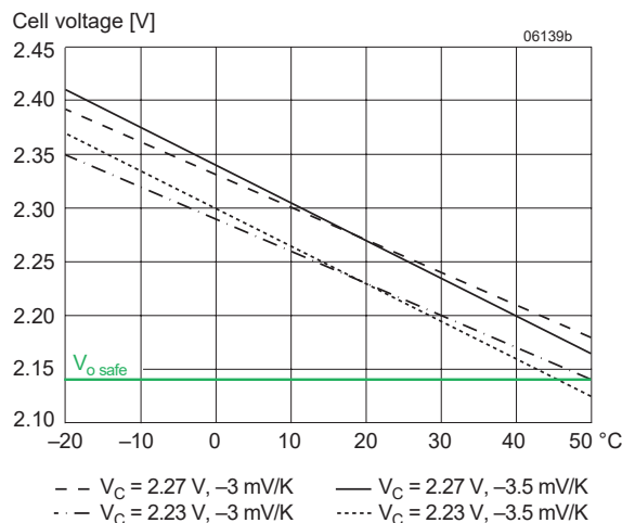
Fig. 20 Trickle charge voltage versus temperature for defined temp. coefficient. V_{o\text{ nom}} is the output voltage with open R-input.
