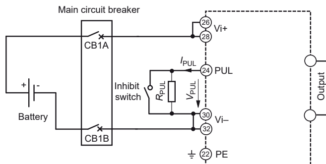
Fig. 16 Circuit for the inhibit function
