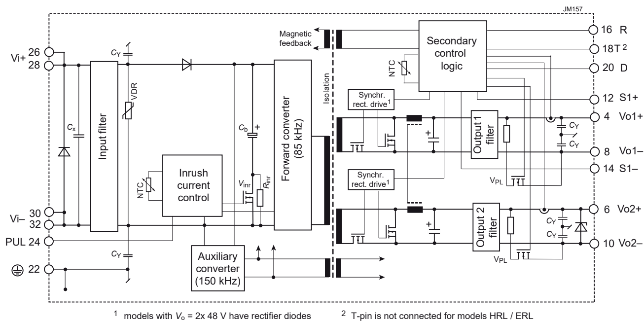
Fig. 2 Block diagram of ER2320
