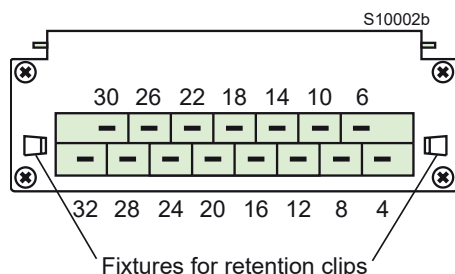
Fig. 29 View of module's male connectors
