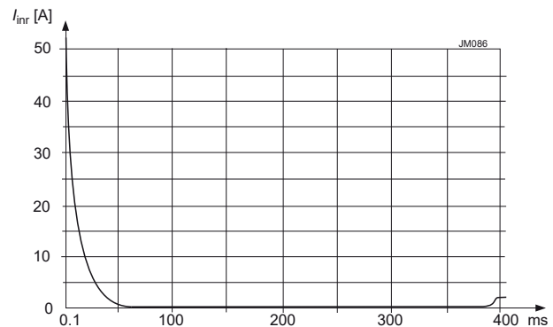
Fig. 7 Inrush current at V_i = 150 \text{ V} , I_{o \text{ nom}} (HR2320, ER2320)
