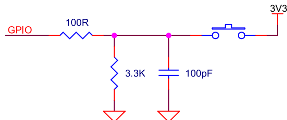
Figure 3 Push-button Strapping for GPIO Pull-down
