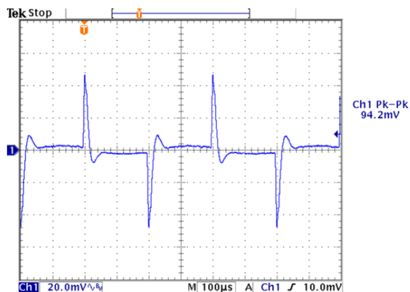
Figure 9. Transient Response without Optimal Voltage Positioning
