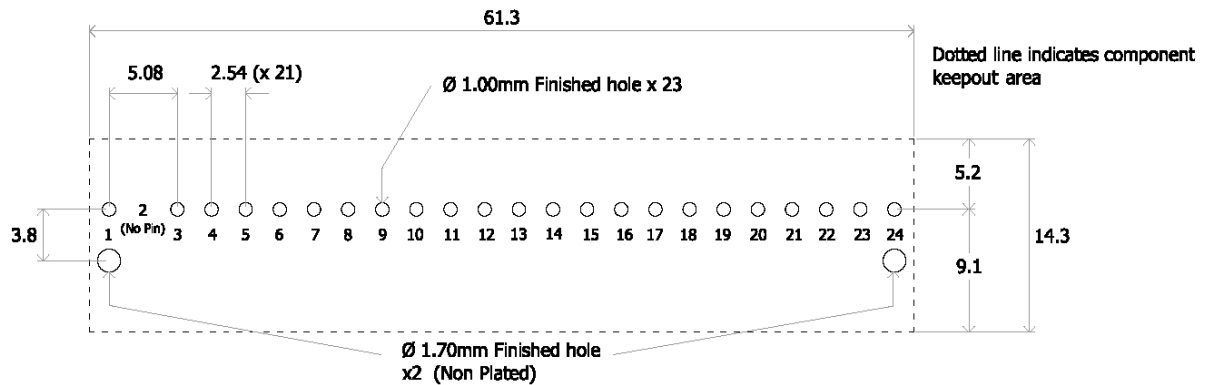
Figure 52. Recommended Footprint – Top View
