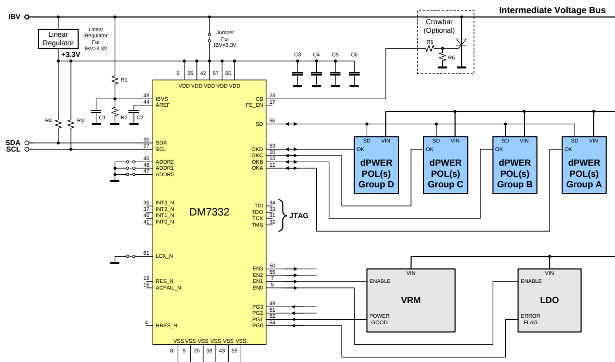
Figure 49. Multi-dPOL Power System Diagram
