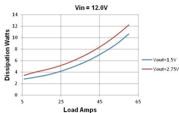
Figure 4. Power Dissipation at Vin = 12V
