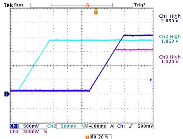
Figure 19. Two outputs delayed 5ms. All slew rates at 0.5V/ms
