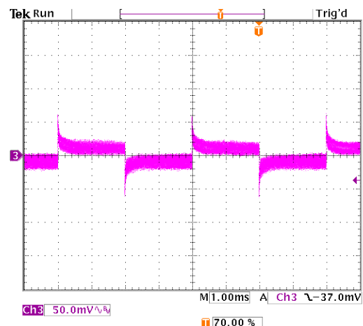
Figure 44. Transient Response with Regulation set to 3.72mV/A
