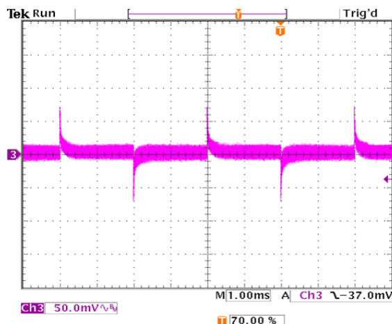
Figure 43. Transient Response with Regulation set to 0.0 mV/A
