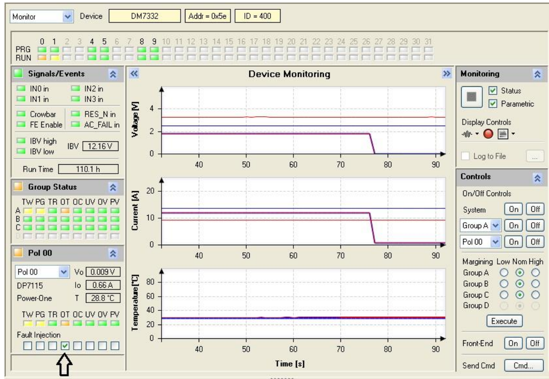
Figure 48. Example Overtemp Fault Injection in the GUI
