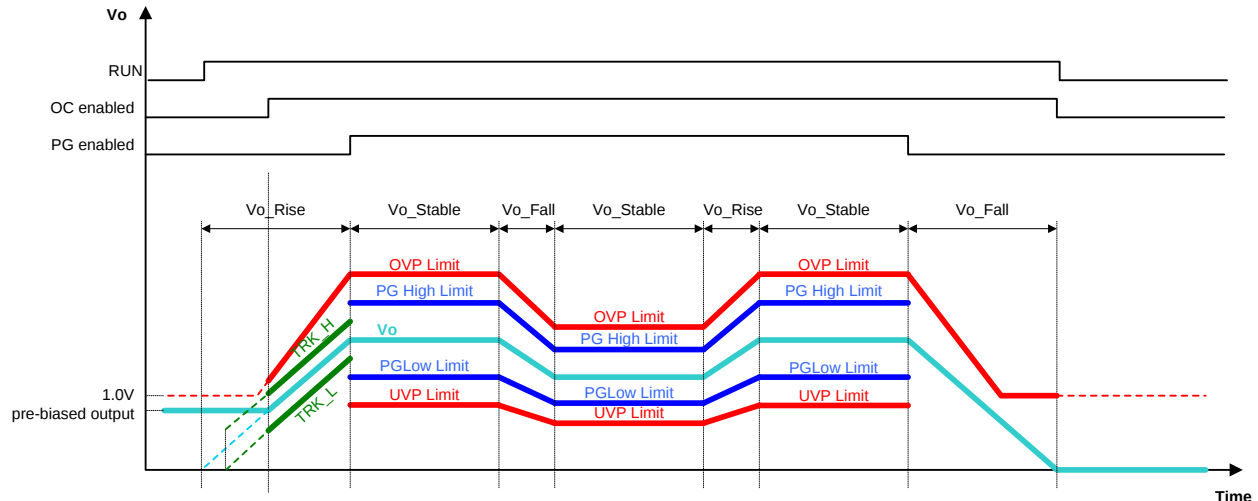
Figure 25. Protections Enable Conditions
