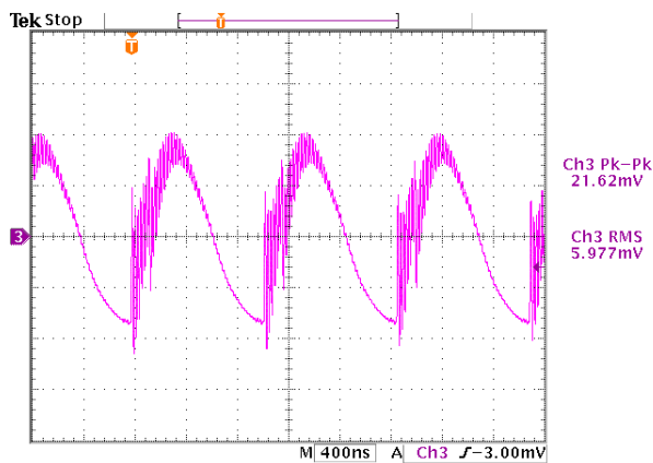
Figure 40. Output Voltage Noise, Full Load, No Interleave
