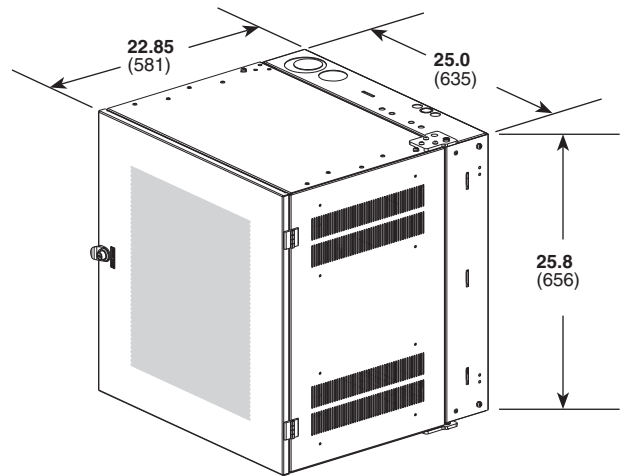
PZC12P – Wall Mount Cabinet with perforated door
