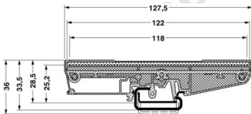
Dimensioned drawing
