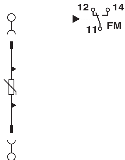
Circuit diagram
