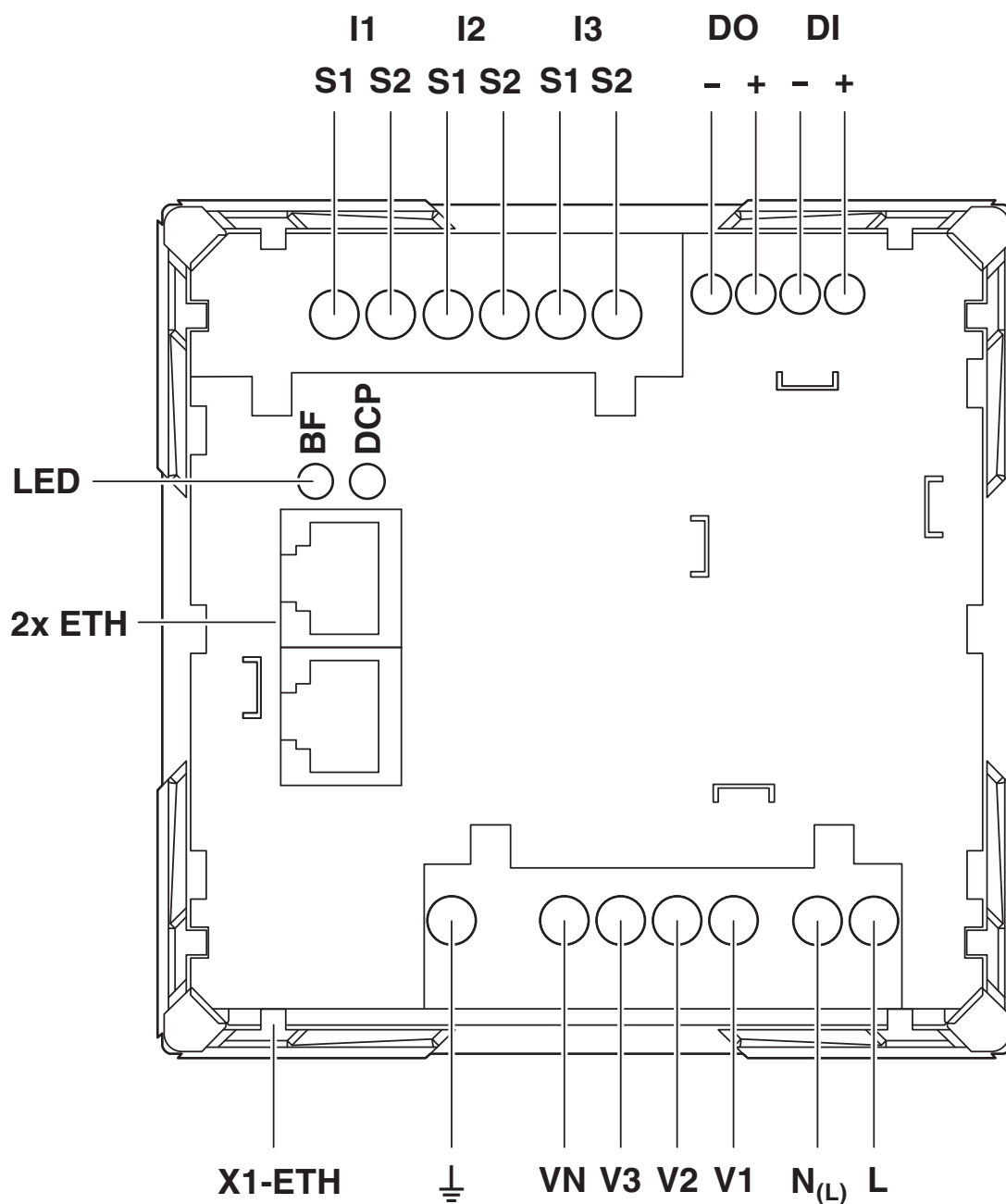
Connection assignment
