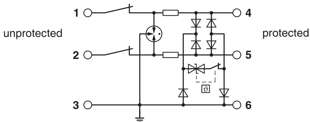
Circuit diagram
