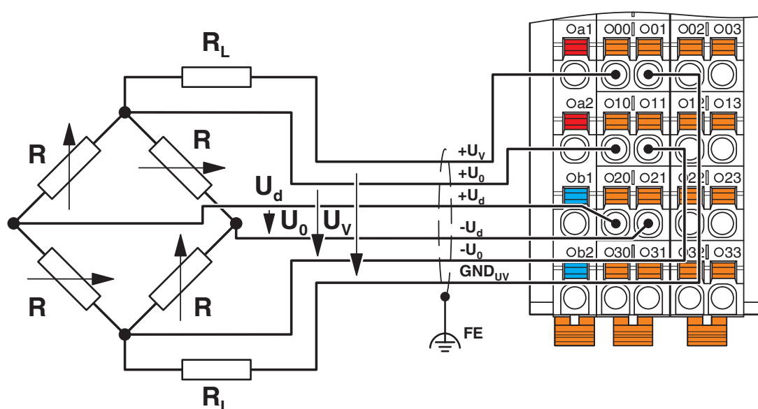
Connection diagram
