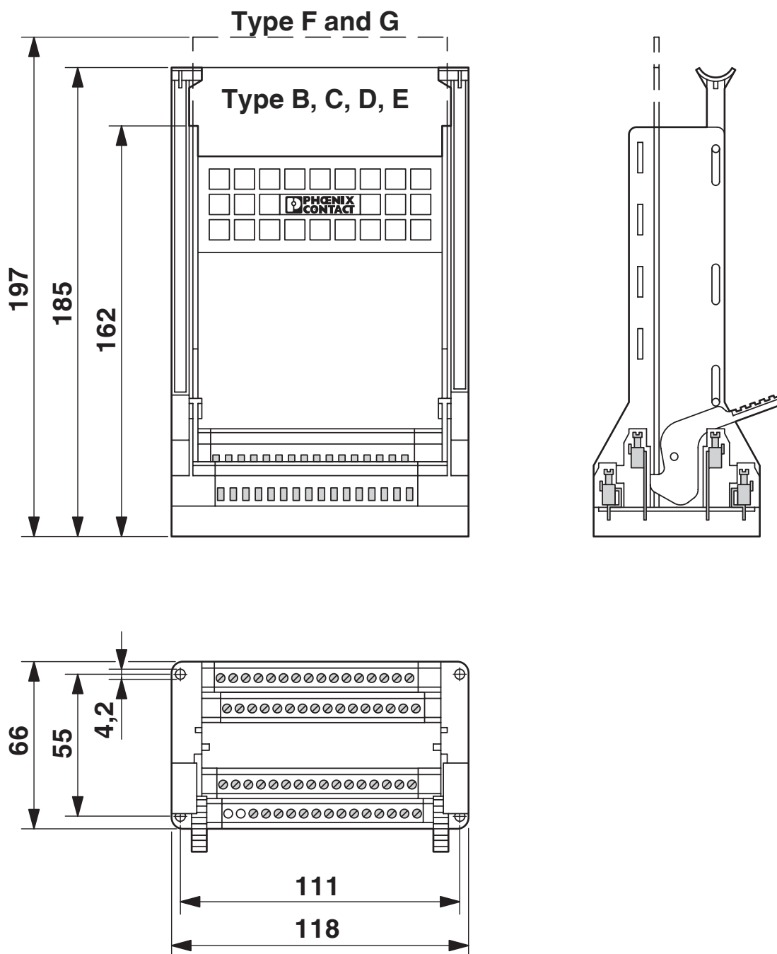
Dimensional drawing
