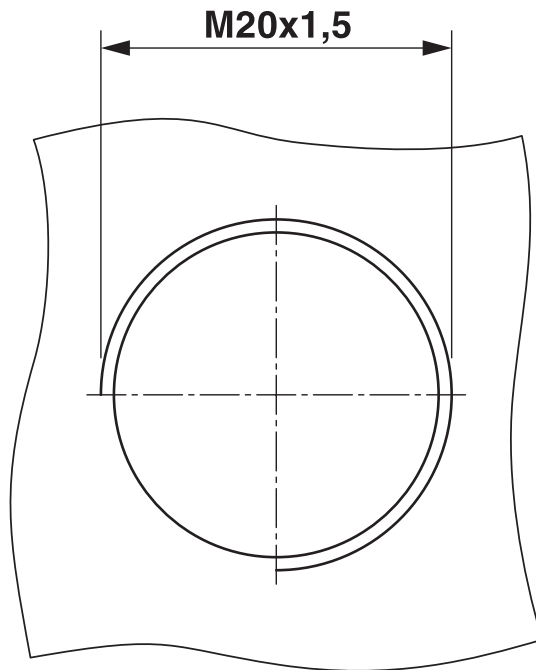
Dimensional drawing
