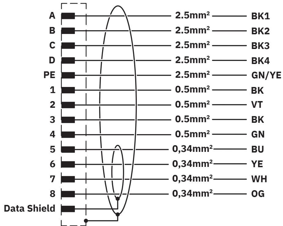
Circuit diagram
