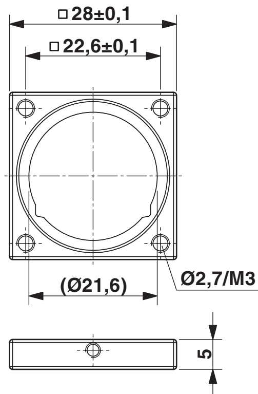
Dimensional drawing
