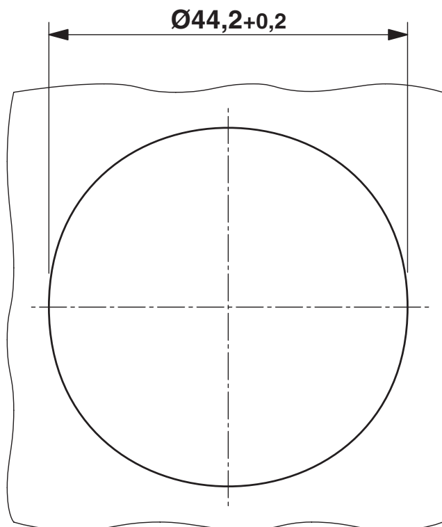
Dimensional drawing
